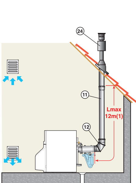
Configuration C33 - Ventouse verticale concentrique
